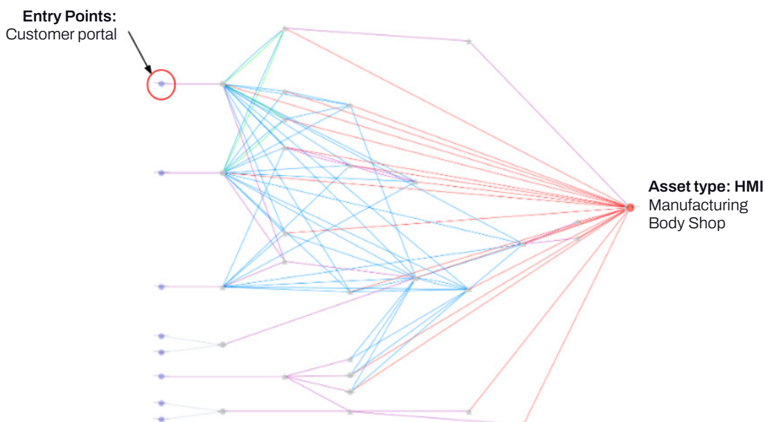
Fig 1: The Armris attack graph is a specialized OT network graph representing the potential attack paths within the network. It identifies the ways an attacker could move through the network to compromise critical assets. The attack graph is based on a powerful, AI based engine that extracts actionable insights based on network topology and traffic flow.
